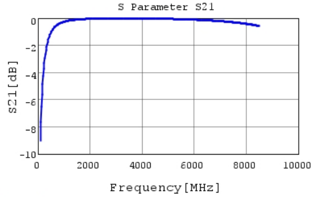
GCQ1555C1H6R0BB01 S21 DCOV, 25degC
