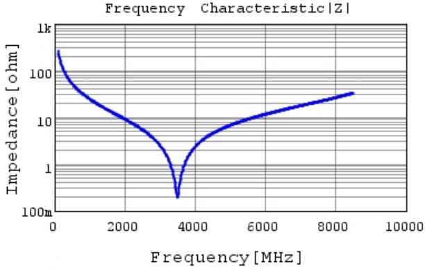
GCQ1555C1H6R0BB01 |Z| DC0V, 25degC
