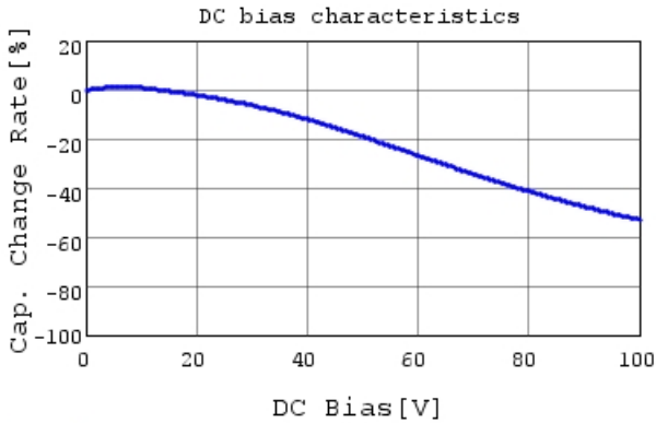
GCD188R72A562MA01 C-DC bias capchange, 25.0c
