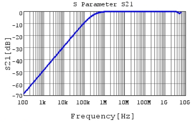
GCD188R72A562MA01 S21 DC0V, 25degC
