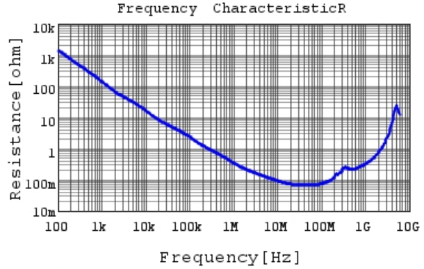
GCD188R72A562MA01 R DCOV, 25degC
