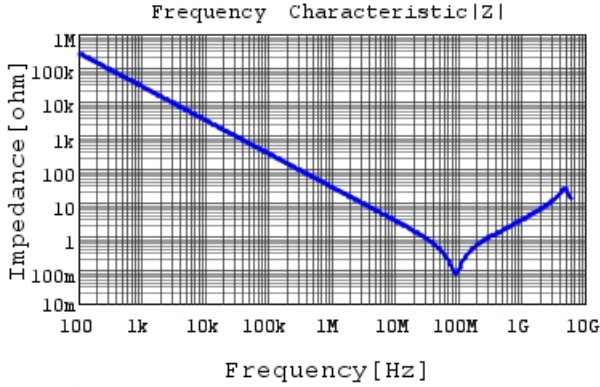
GCD188R72A562MA01 |Z| DCOV, 25degC
