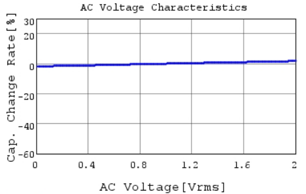
GCD188R72A562MA01 C-AC Voltage capchange, Dc
