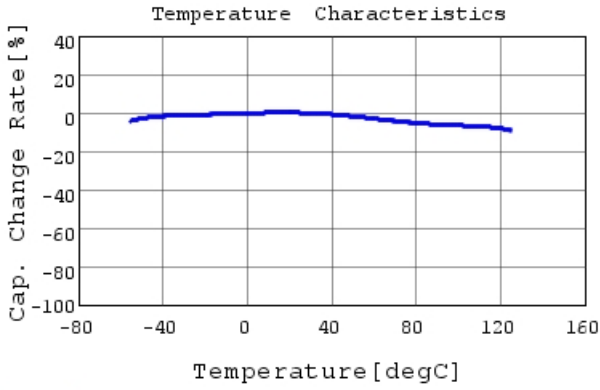
GCD188R72A562MA01 C-Temp. capchange, DC0.0V,
