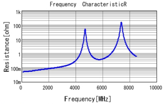
GQM1875C2E150GB12 R DCOV, 25degC
