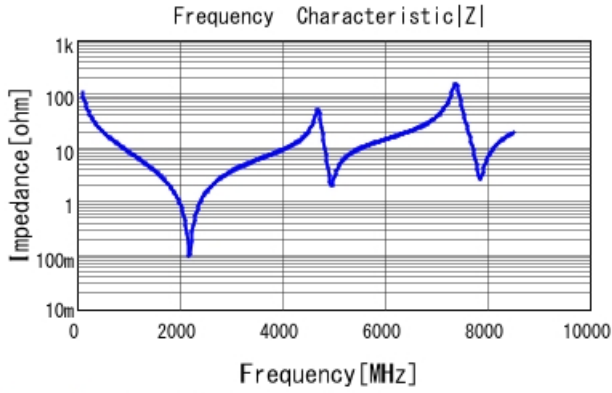
GQM1875C2E150GB12 |Z| DCOV, 25degC
