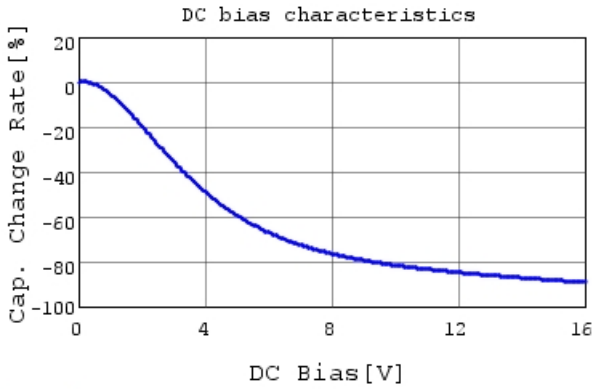
GRT188C81C106ME13 C-DC bias capchange, 25.0c
