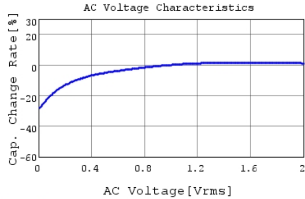
GRT188C81C106ME13 C-AC Voltage capchange, Dc
