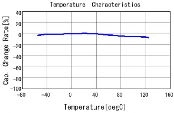
■ GCD188R71H682KA01 C-Temp. capchange, DCO. 0V, AC1. 0Vrm
