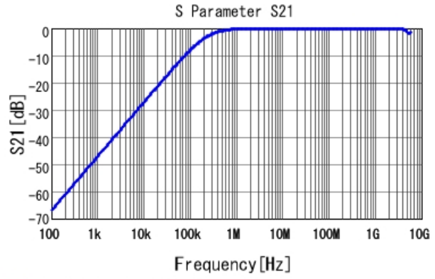
■ GCD188R71H682KA01 S21 DCOV, 25degC
