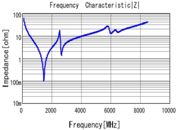
■ GQM1885C1H270JB01 |Z| DC0V, 25degC
