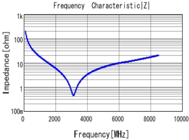
■ GRM1552C1H8R0CA01 |Z| DCOV, 20degC
