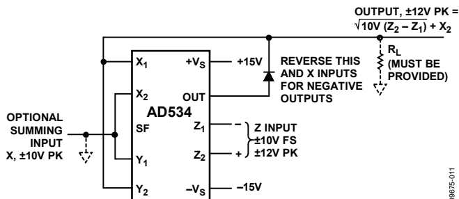
Figure 19. Square-Rooter Connection
