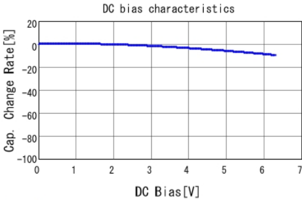
GRM155R60J104KA01 C-DC bias capchange, 25.0degC, A
