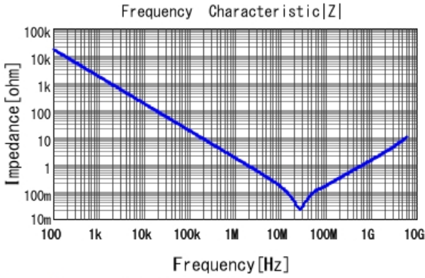
GRM155R60J104KA01 |Z| DCOV, 25degC
