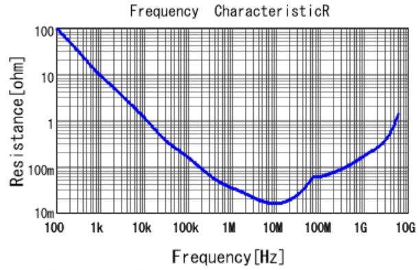
GRM155R60J104KA01 R DCOV, 25degC
