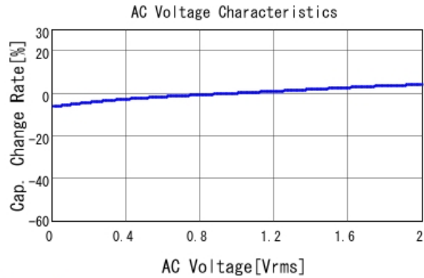
GRM155R60J104KA01 C-AC Voltage capchange, DCOV, 25
