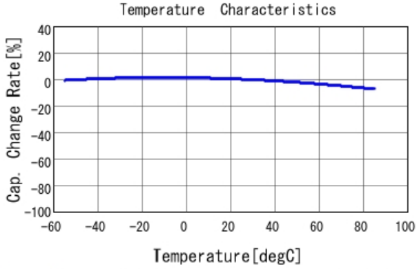
GRM155R60J104KA01 C-Temp. capchange, DC0.0V, AC1.C
