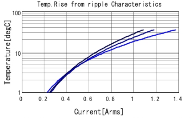
GRM1555C1H101GA01 Temp. rise — 200MHz — 500I
