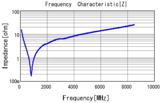
GRM1555C1H101GA01 |Z| DCOV, 25degC
