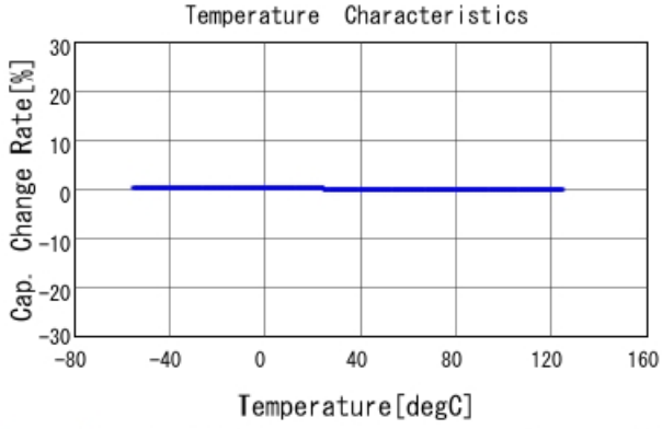
GRM1555C1H101GA01 C-Temp. capchange, DCOV, AC1Vrms
