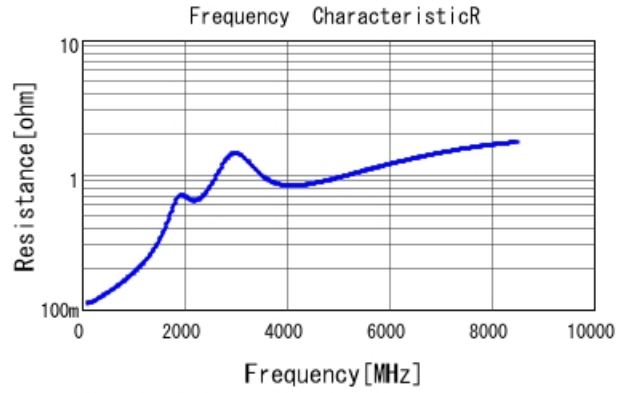
GRM1555C1H101GA01 R DCOV, 25degC
