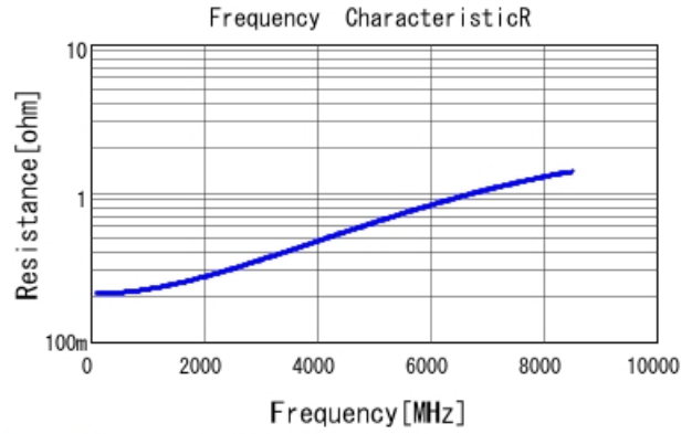
GRM0335C1E5R0BA01 R DCOV, 25degC
