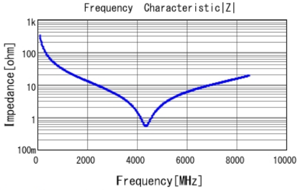
GRM0335C1E5R0BA01 |Z| DCOV, 25degC
