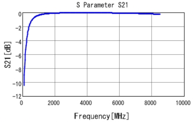
GRM0335C1E5R0BA01 S21 DCOV, 25degC
