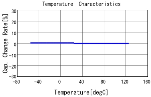
GRM0335C1E5R0BA01 C-Temp. capchange, DCOV, AC1Vrms
