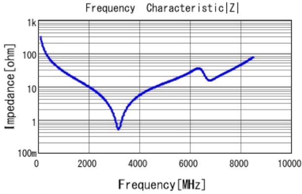
GRM1885C1H5R1WA01 |Z| DCOV, 25degC
