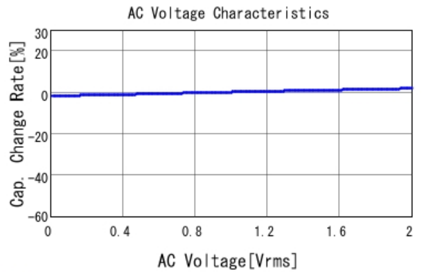
GCD188R72A822MA01 C-AC Voltage capchange, DCOV, 25.0d
