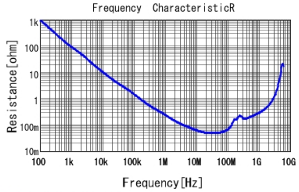
GCD188R72A822MA01 R DCOV, 25degC
