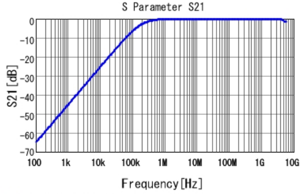
■ GCD188R72A822MA01 S21 DCOV, 25degC
