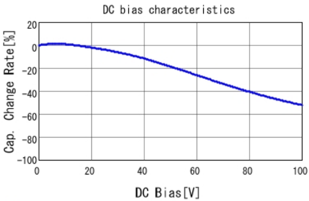
GCD188R72A822MA01 C-DC bias capchange, 25.0degC, AC1.
