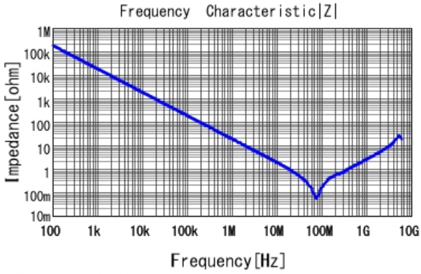
GCD188R72A822MA01 |Z| DCOV, 25degC
