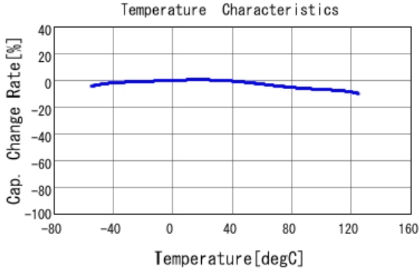
■ GCD188R72A822MA01 C-Temp. capchange, DCO. 0V, AC1. 0Vrm
