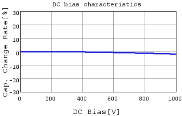
GRM31C7U3A102JW32 C-DC bias capchange, 25.0c
