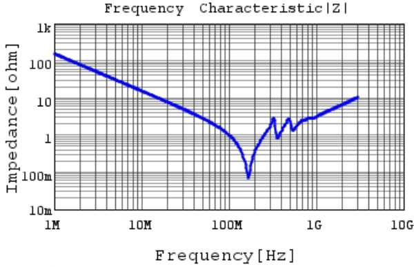
GRM31C7U3A102JW32 |Z| DC0V, 25degC
