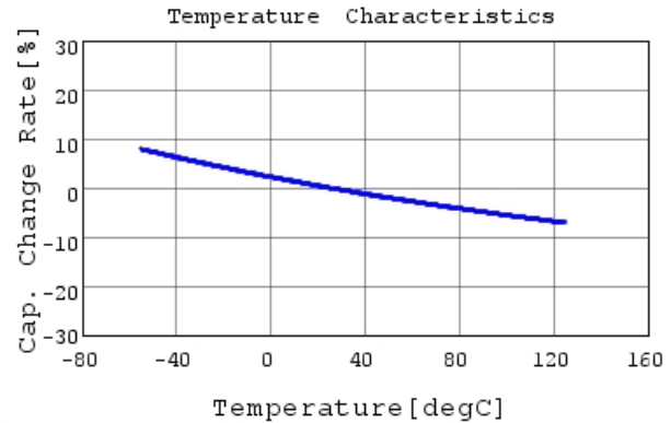
GRM31C7U3A102JW32 C-Temp. capchange, DC0V, 1
