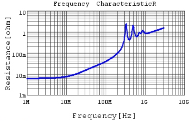
GRM31C7U3A102JW32 R DC0V, 25degC
