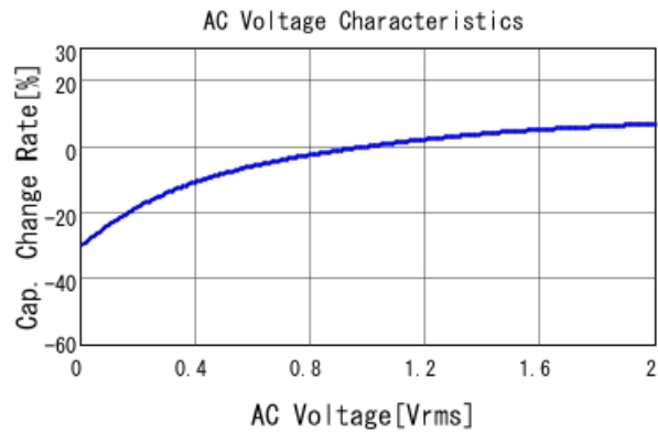
■ GCJ21BC71C106KE02 C-AC Voltage capchange, DC0V, 25.0d
