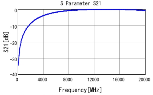
GRM1555C1HR30WA01 S21 DCOV, 25degC
