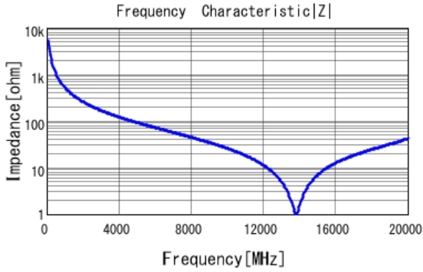
GRM1555C1HR30WA01 |Z| DCOV, 25degC
