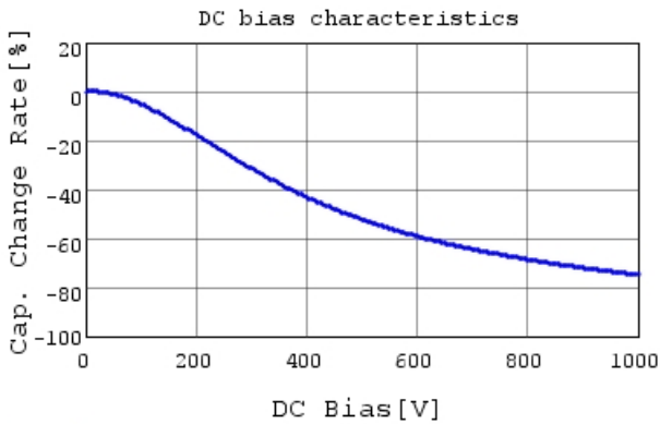
GCJ31BR73A222KXJ1 C-DC bias capchange, 25.0c
