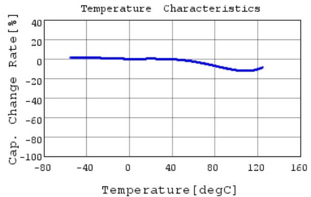
GCJ31BR73A222KXJ1 C-Temp. capchange, DCOV, 1
