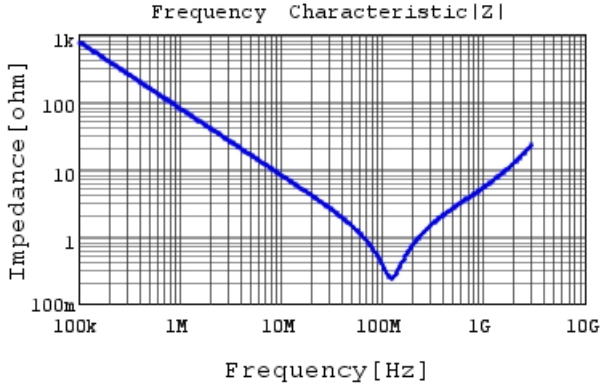
GCJ31BR73A222KXJ1 |Z| DCOV, 25degC
