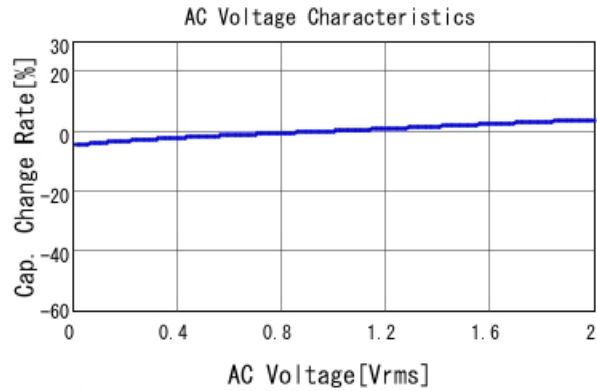
GRM188B31E224KA87 C-AC Voltage capchange, DCOV, 2C
