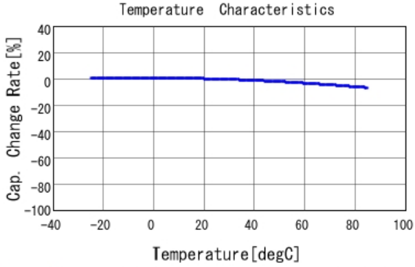
GRM188B31E224KA87 C-Temp. capchange, DC0.0V, AC1.C
