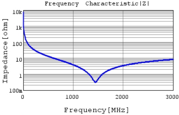
GRM1885C2E220FW07 |Z| DC0V, 25degC
