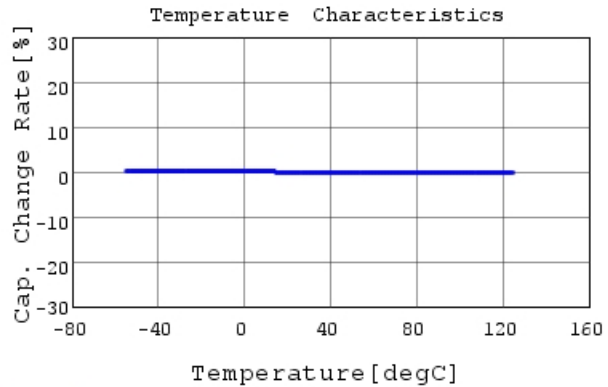
GRM1885C2E220FW07 C-Temp. capchange, DC0V, 1
