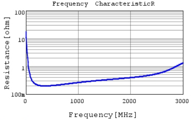
GRM1885C2E220FW07 R DC0V, 25degC
