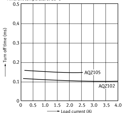
16-4. Turn off time vs. load current characteristics (AC/DC type)
