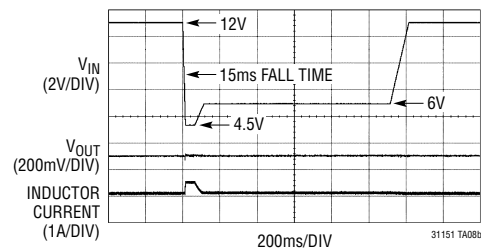
Cold Crank Line Transient with 1A Load
