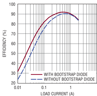
Efficiency vs Load Current VIN = 12V
