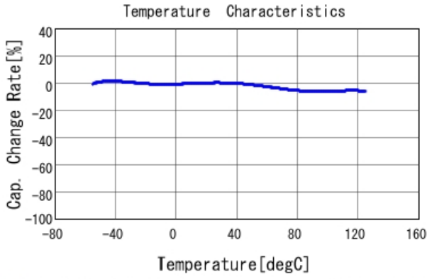
■ GCD188R72A272MA01 C-Temp. capchange, DCO. 0V, AC1. 0V rm
