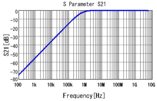
■ GCD188R72A272MA01 S21 DCOV, 25degC
