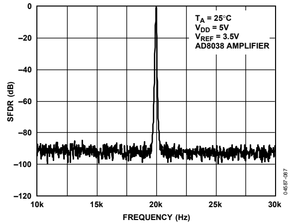
Figure 37. Narrow-Band SFDR, f_{OUT} = 20\text{ kHz} , Clock = 1 MHz
