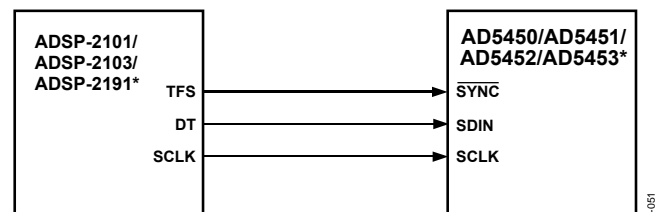
Figure 54. ADSP-2101/ADSP-2103/ADSP-2191* SPORT-to-AD5450/AD5451/AD5452/AD5453 Interface
