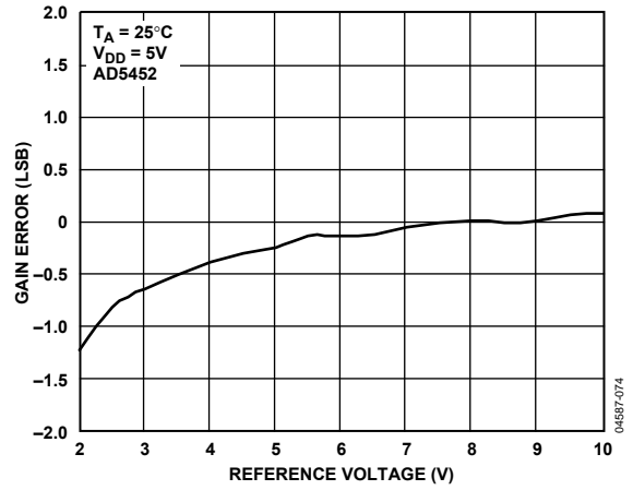
Figure 21. Gain Error (LSB) vs. Reference Voltage
