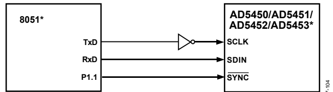
Figure 57. 80C51/80L51-to-AD5450/AD5451/AD5452/AD5453 Interface
