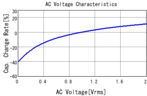
GRM155R61C224MA12 C-AC Voltage capchange, DCOV, 25
