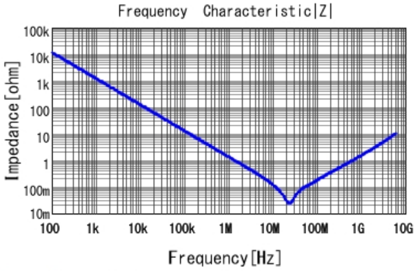
GRM155R61C224MA12 |Z| DCOV, 25degC
