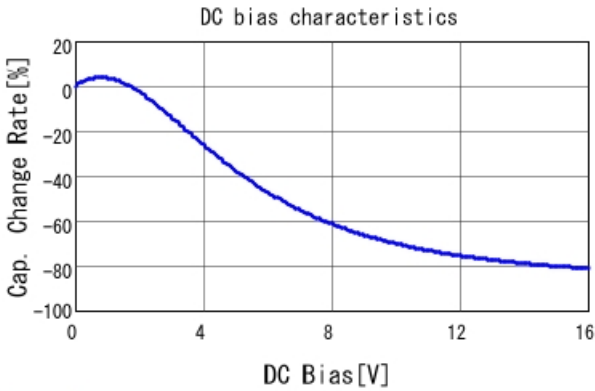
GRM155R61C224MA12 C-DC bias capchange, 25.0degC, A
