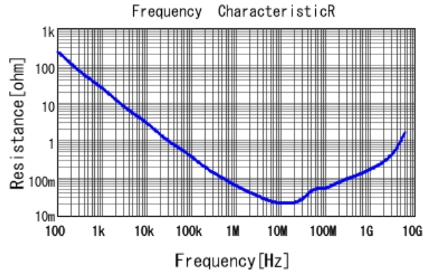
GRM155R61C224MA12 R DCOV, 25degC
