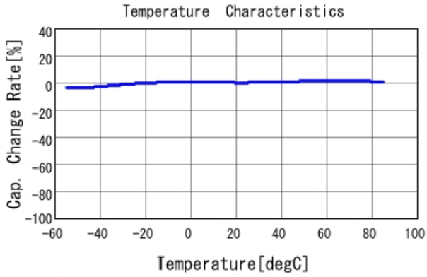
GRM155R61C224MA12 C-Temp. capchange, DC0.0V, AC1.C
