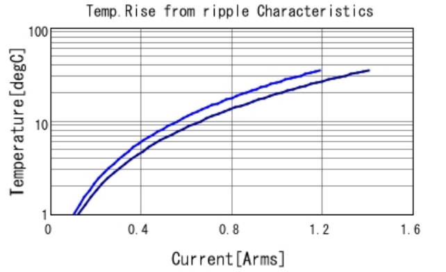
GRM155R61C224MA12 Temp. rise — 600kHz — 1MHz
