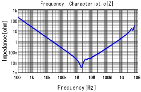
GRM32DR61C106KA01 |Z| DCOV, 25degC
