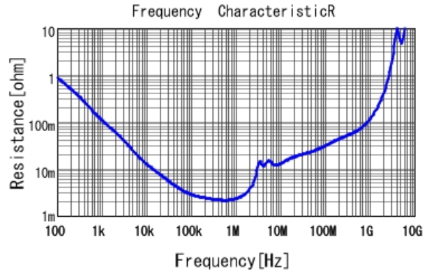
GRM32DR61C106KA01 R DCOV, 25degC
