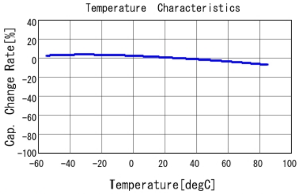
GRM32DR61C106KA01 C-Temp. capchange, DC0.0V, AC1.C
