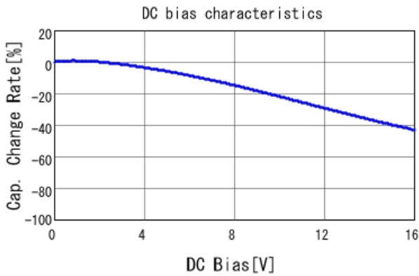
GRM32DR61C106KA01 C-DC bias capchange, 25.0degC, A
