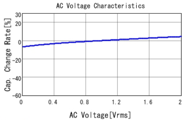
GRM32DR61C106KA01 C-AC Voltage capchange, DCOV, 25
