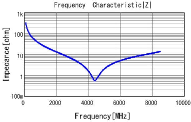
GRM0335C2A4R8WA01 |Z| DCOV, 25degC
