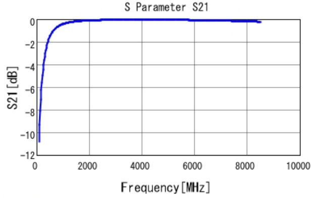
GRM0335C2A4R8WA01 S21 DCOV, 25degC
