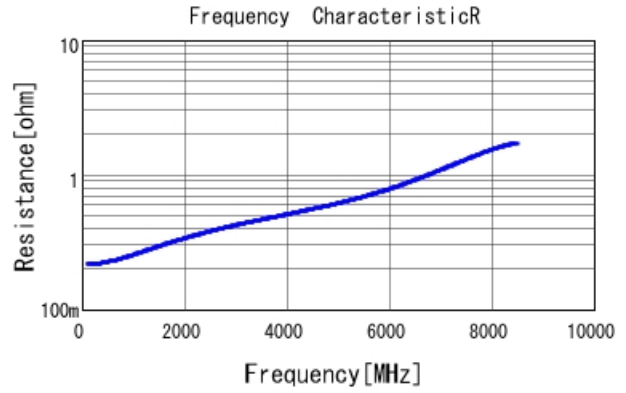
GRM0335C2A4R8WA01 R DCOV, 25degC
