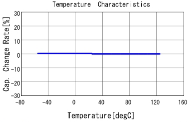
GRM0335C2A4R8WA01 C-Temp. capchange, DCOV, AC1Vrms
