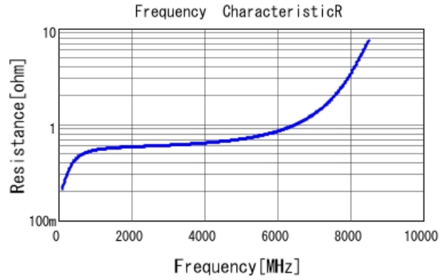
GRM1885C1H1R5CA01 R DCOV, 25degC
