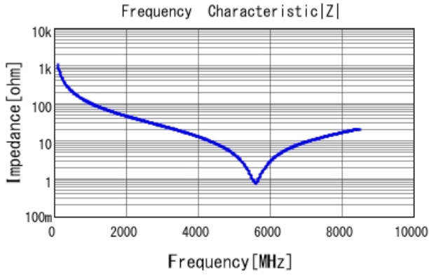
GRM1885C1H1R5CA01 |Z| DCOV, 25degC
