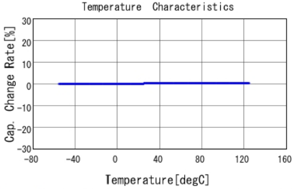
GRM1885C1H1R5CA01 C-Temp. capchange, DC0V, AC1Vrms
