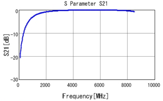
GRM1885C1H1R5CA01 S21 DC0V, 25degC
