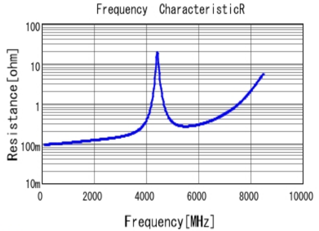
■ GQM1885C1H8R2DB01 R DCOV, 25degC
