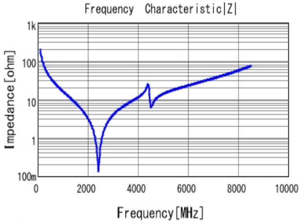
■ GQM1885C1H8R2DB01 |Z| DCOV, 25degC
