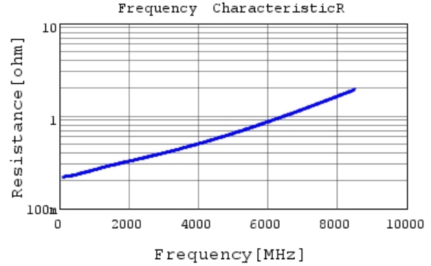
GRM0335C2A4R6CA01 R DCOV, 25degC
