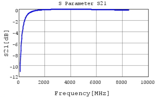
GRM0335C2A4R6CA01 S21 DCOV, 25degC
