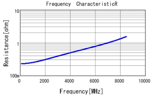
■ GRM0335C2A4R1WA01 R DCOV, 25degC
