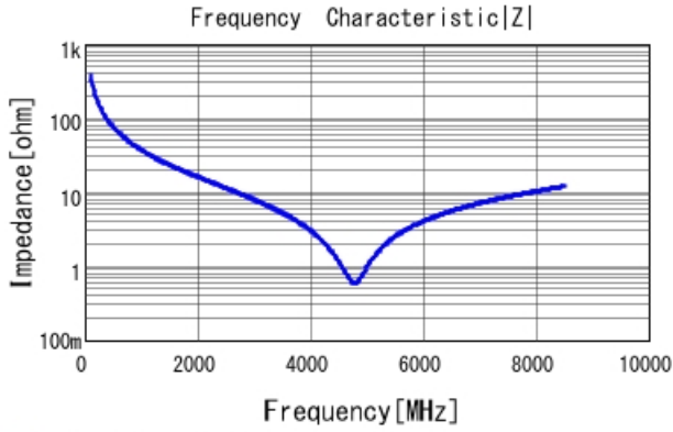
■ GRM0335C2A4R1WA01 |Z| DCOV, 25degC
