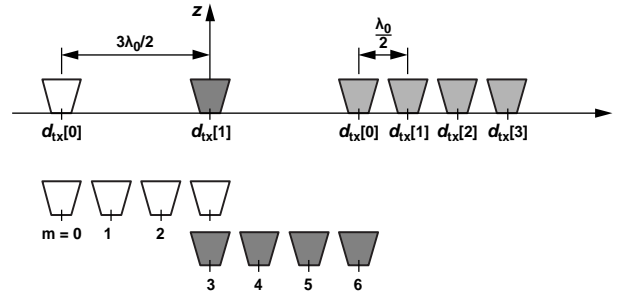
Figure 6. Antenna Arrangement with Virtual Antenna Positions
