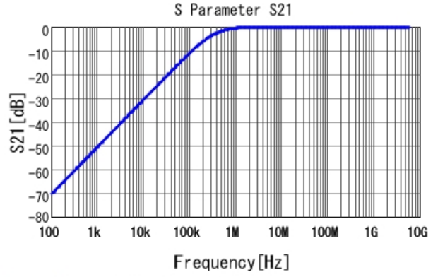
GRM155R61E472KA01 S21 DC0V, 25degC
