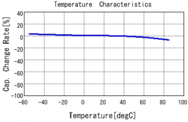
GRM155R61E472KA01 C-Temp. capchange, DC0.0V, AC1.C
