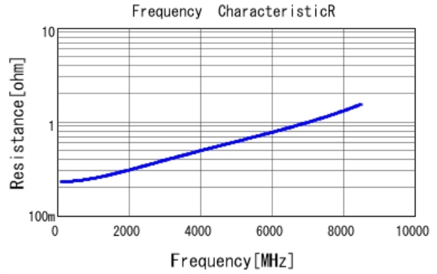
■ GRM0335C2A4R1CA01 R DCOV, 25degC
