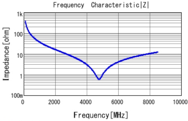
■ GRM0335C2A4R1CA01 |Z| DCOV, 25degC
