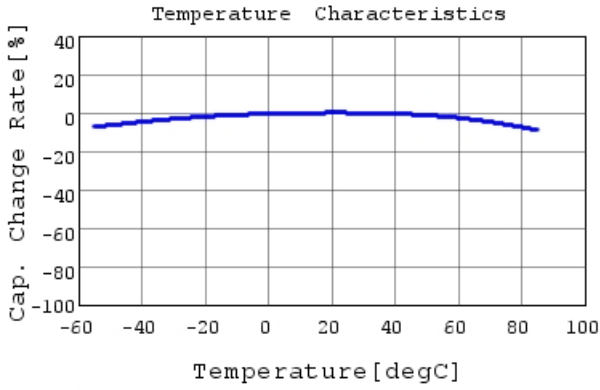
GRM033R61A153ME84 C-Temp. capchange, DC0.0V,
