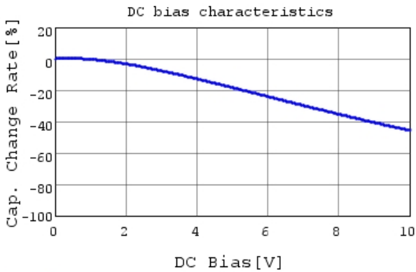
GRM033R61A153ME84 C-DC bias capchange, 25.0c
