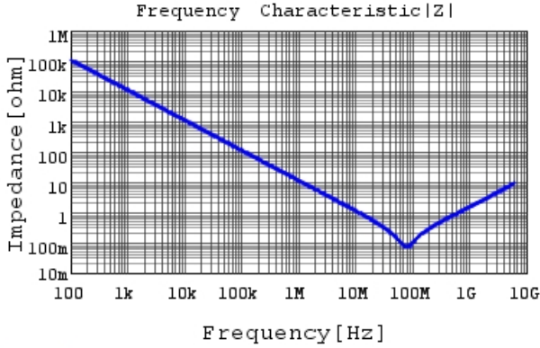
GRM033R61A153ME84 |Z| DCOV, 25degC
