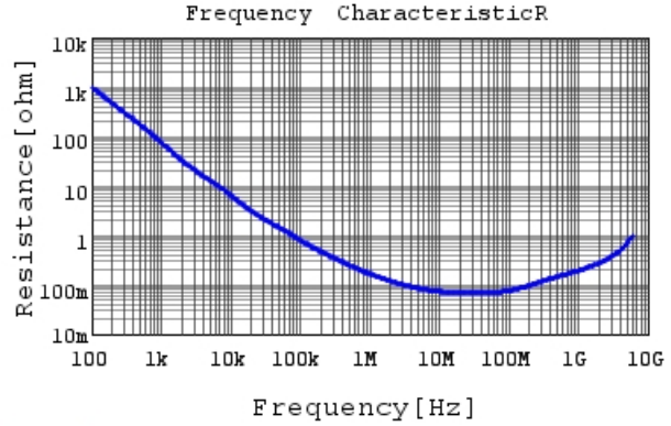
GRM033R61A153ME84 R DCOV, 25degC
