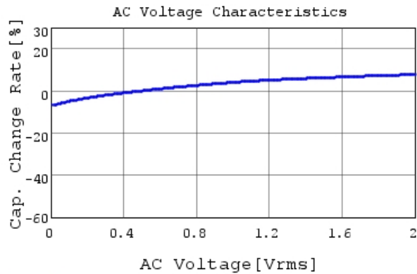
GRM033R61A153ME84 C-AC Voltage capchange, Dc
