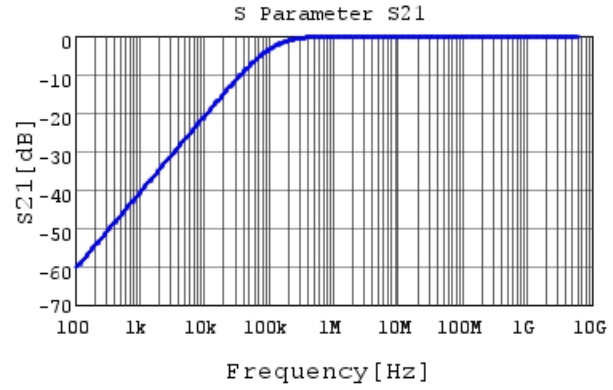
GRM033R61A153ME84 S21 DC0V,25degC
