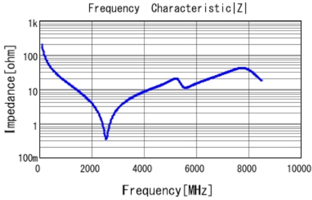
GCM1885C1H8R2DA16 |Z| DCOV, 25degC
