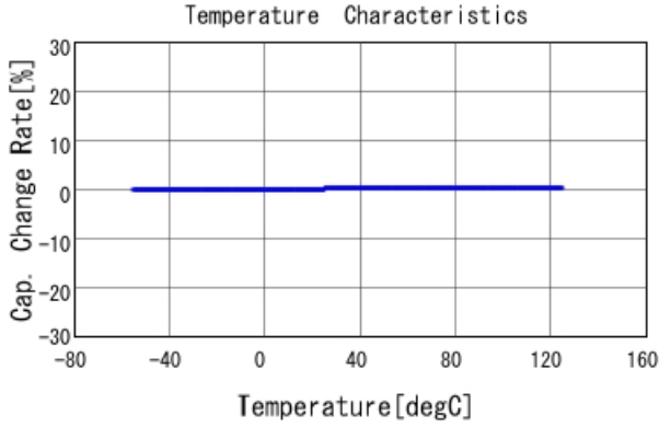
GCM1885C1H8R2DA16 C-Temp. capchange, DCOV, AC1Vrms
