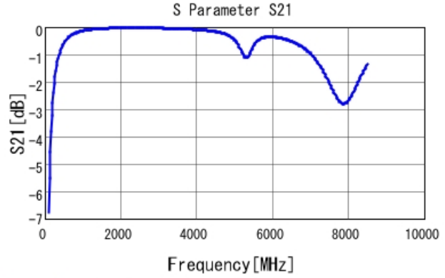
GCM1885C1H8R2DA16 S21 DCOV, 25degC
