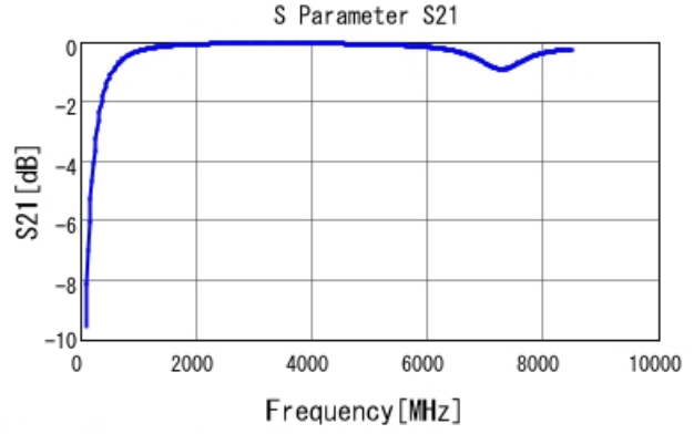
GRM1555C1H5R6CA01 S21 DCOV, 25degC
