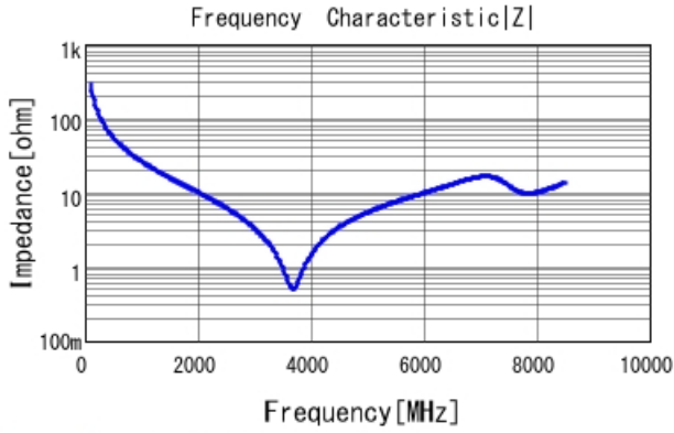
GRM1555C1H5R6CA01 |Z| DCOV, 25degC
