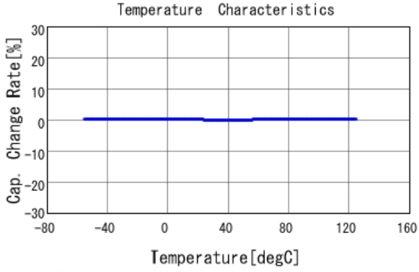
GRM1555C1H5R6CA01 C-Temp. capchange, DCOV, AC1Vrms
