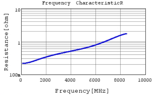
GRM0335C2A4R7WA01 R DC0V, 25degC
