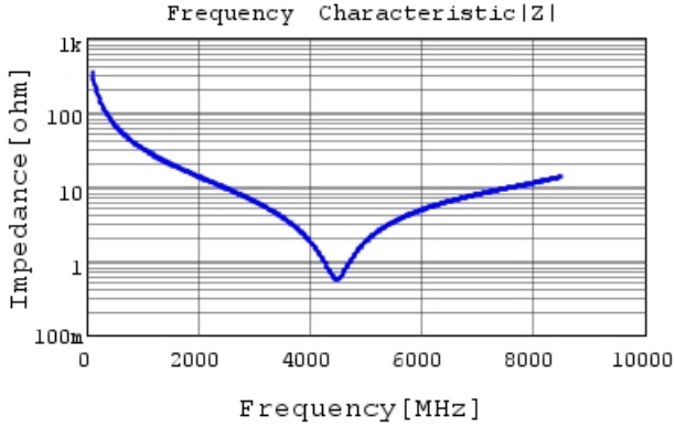
GRM0335C2A4R7WA01 |Z| DC0V, 25degC
