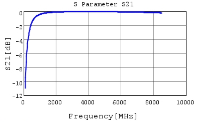
GRM0335C2A4R7WA01 S21 DCOV, 25degC
