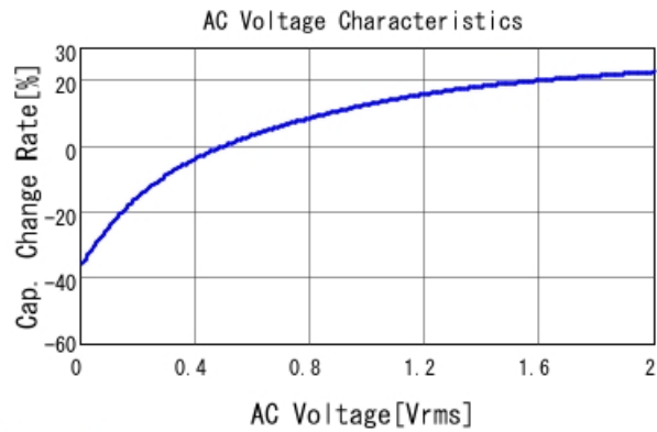
GRJ188R70J225KE11 C-AC Voltage capchange, DCOV, 25
