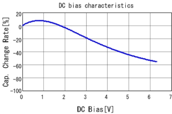
GRJ188R70J225KE11 C-DC bias capchange, 25.0degC, A
