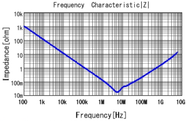
GRJ188R70J225KE11 |Z| DCOV, 25degC
