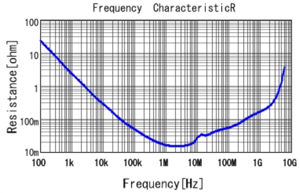
GRJ188R70J225KE11 R DCOV, 25degC
