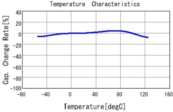
GRJ188R70J225KE11 C-Temp. capchange, DC0.0V, AC0.5
