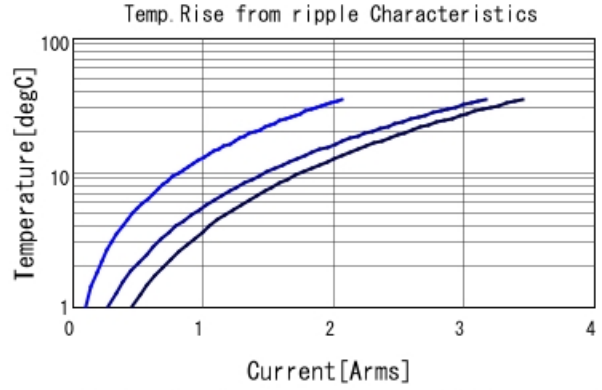
GRJ188R70J225KE11 Temp. rise — 100kHz — 500
