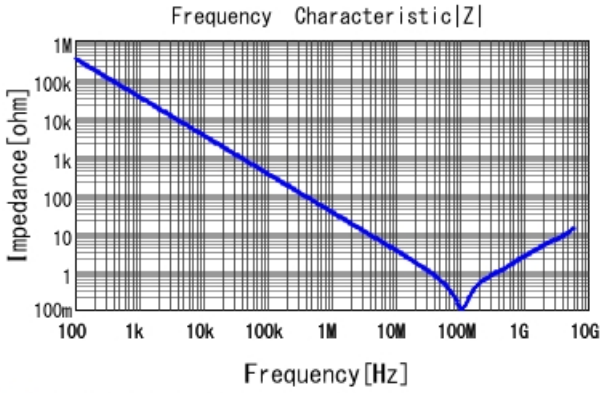
GCD188R71H472KA01 |Z| DCOV, 25degC
