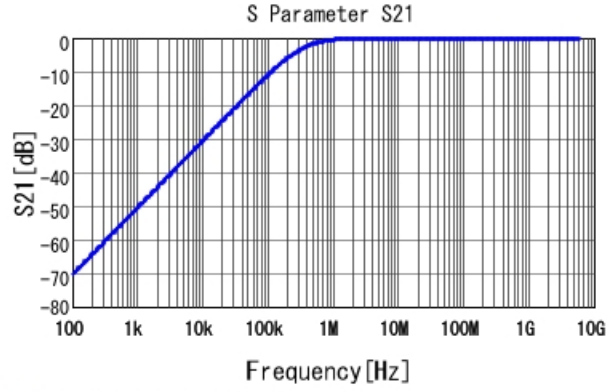
■ GCD188R71H472KA01 S21 DCOV, 25degC
