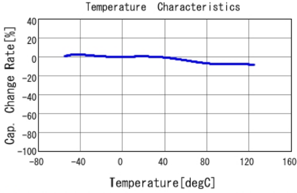
■ GCD188R71H472KA01 C-Temp. capchange, DCO. 0V, AC1. 0Vrm
