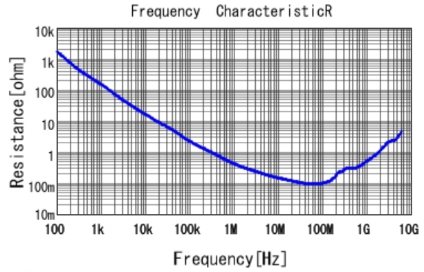
GCD188R71H472KA01 R DCOV, 25degC
