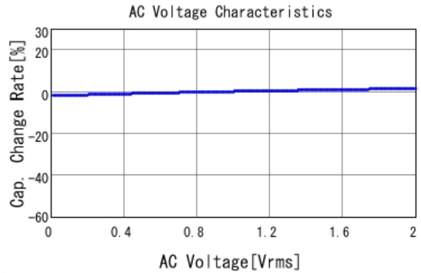
GCD188R71H472KA01 C-AC Voltage capchange, DCOV, 25.0d
