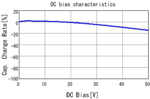
GCD188R71H472KA01 C-DC bias capchange, 25.0degC, AC1.
