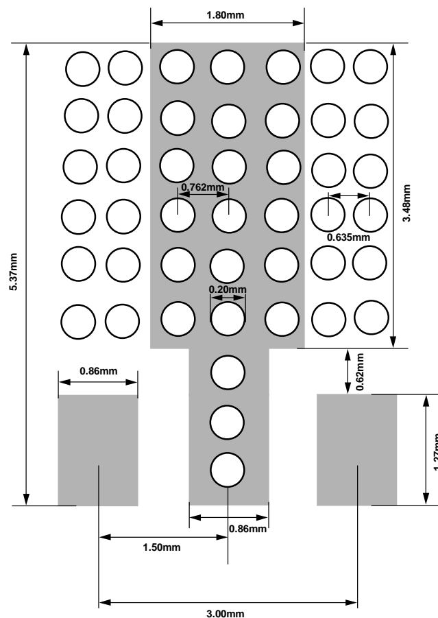
Figure 35. Recommended Land Pattern
