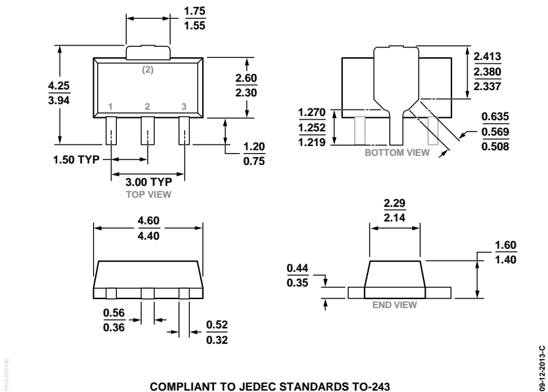
Figure 47. 3-Lead Small Outline Transistor Package [SOT-89] (RK-3) Dimensions shown in millimeters
