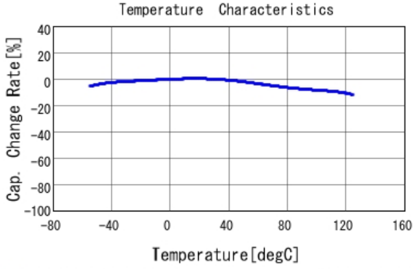
■ GCD21BR71H823MA01 C-Temp. capchange, DCO. 0V, AC1. 0Vrm
