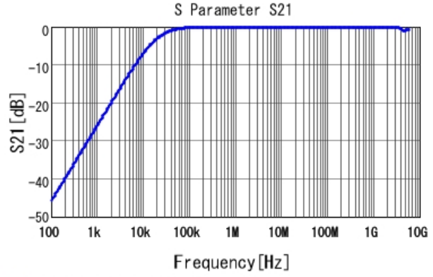
■ GCD21BR71H823MA01 S21 DCOV, 25degC
