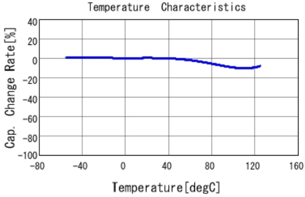
GRM21BR72A473MA01 C-Temp. capchange, DC0.0V, AC1.C
