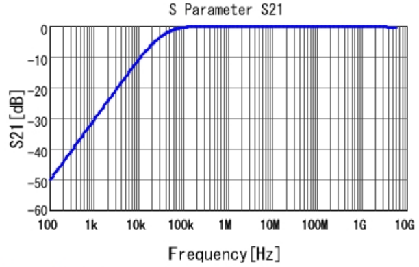
GRM21BR72A473MA01 S21 DC0V, 25degC
