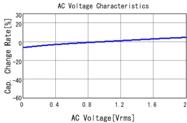
GCJ188R71C334KA01 C-AC Voltage capchange, DCOV, 25
