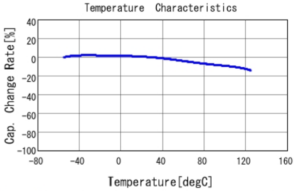
GCJ188R71C334KA01 C-Temp. capchange, DC0.0V, AC1.C
