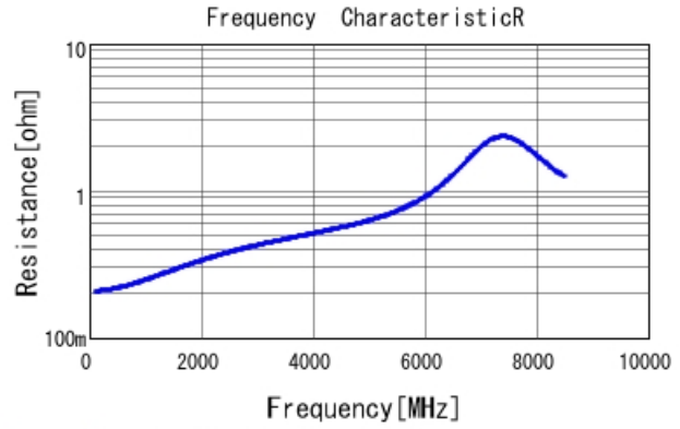
GRM1555C1H6R3CA01 R DCOV, 25degC
