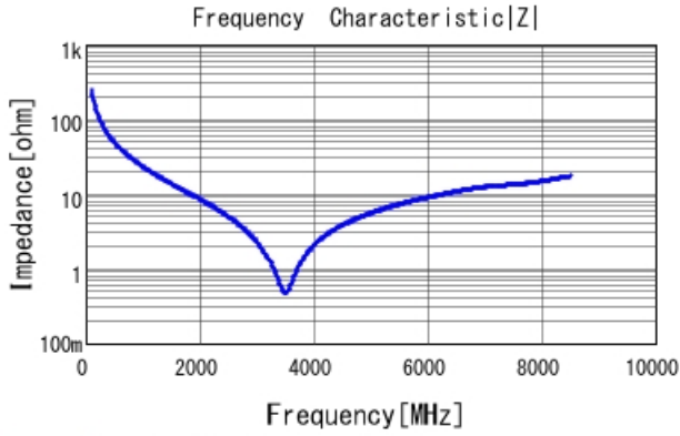
GRM1555C1H6R3CA01 |Z| DCOV, 25degC
