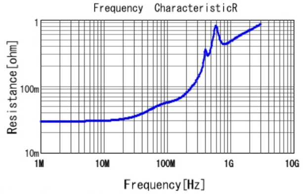
GCM21A7U2E102JX01 R DCOV, 25degC
