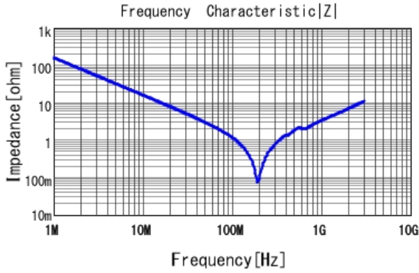
GCM21A7U2E102JX01 |Z| DCOV, 25degC
