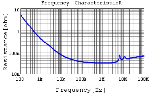
RDEC72A225K3K1H03B R DC0V, 25degC
