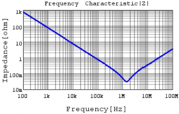
RDEC72A225K3K1H03B |Z| DC0V, 25degC
