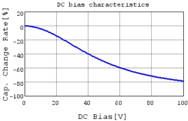
RDEC72A225K3K1H03B C-DC bias capchange, 25.0
