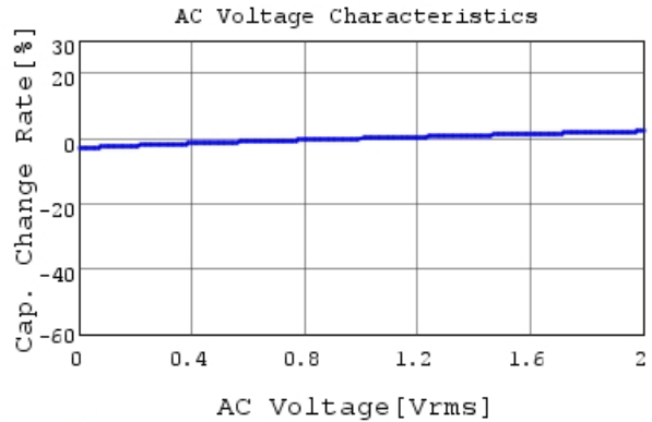
RDEC72A225K3K1H03B C-AC Voltage capchange, I
