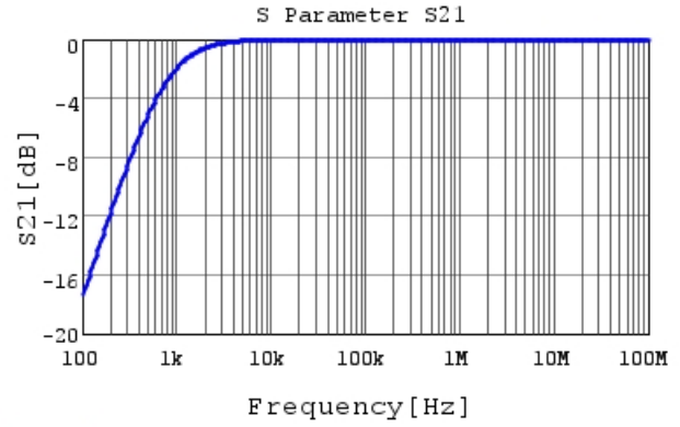
RDEC72A225K3K1H03B S21 DC0V, 25degC
