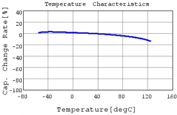
RDEC72A225K3K1H03B C-Temp. capchange, DC0.0V
