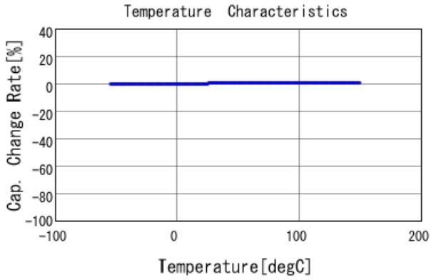
GQM2195G2H3R0CB12 C-Temp. capchange, DCOV, AC1Vrms
