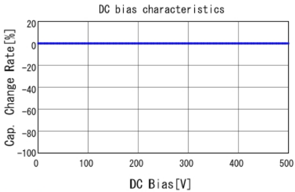
GQM2195G2H3R0CB12 C-DC bias capchange, 25.0degC, A
