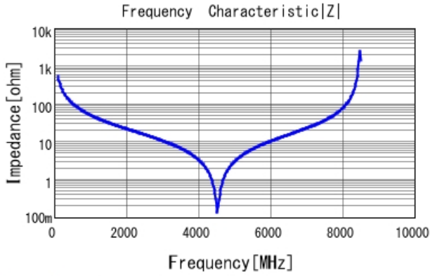
GQM2195G2H3R0CB12 |Z| DCOV, 25degC
