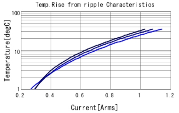
GQM2195G2H3R0CB12 Temp. rise — 1GHz — 2GHz
