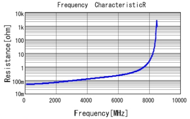
GQM2195G2H3R0CB12 R DCOV, 25degC
