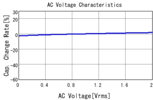
GCJ216R71H223KA01 C-AC Voltage capchange, DCOV, 25
