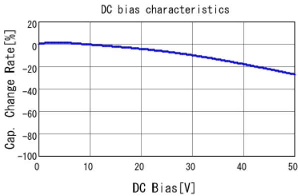
GCJ216R71H223KA01 C-DC bias capchange, 25.0degC, A
