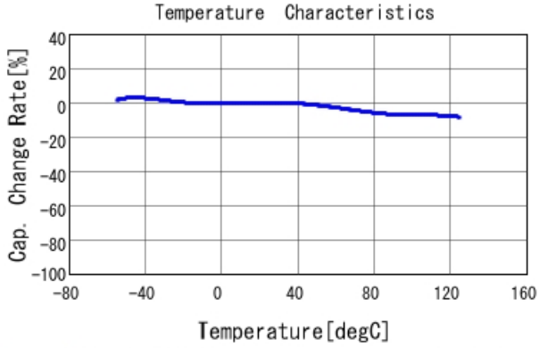
GCJ216R71H223KA01 C-Temp. capchange, DC0.0V, AC1.C
