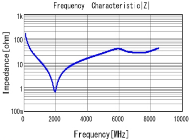
■ GRT1885C2A100JA02 |Z| DC0V, 25degC
