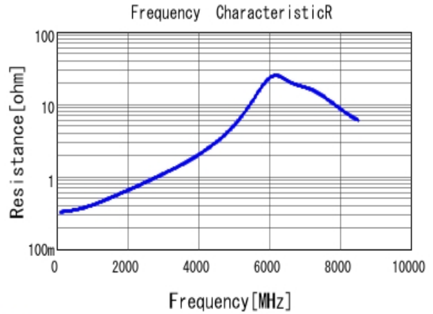
■ GRT1885C2A100JA02 R DC0V, 25degC
