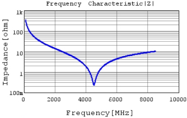
GJM0335C1E4R6CB01 |Z| DC0V, 25degC
