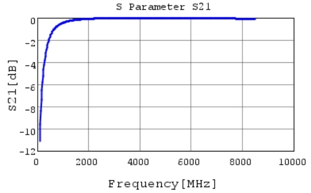
GJM0335C1E4R6CB01 S21 DCOV, 25degC
