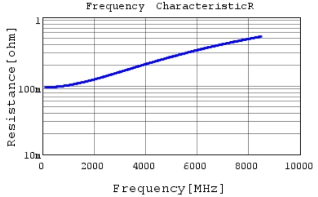
GJM0335C1E4R6CB01 R DC0V, 25degC
